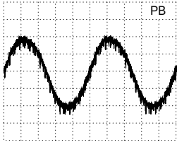
AC, 200mV/Div, 200µs/Div IC7608-(7) ⑧
