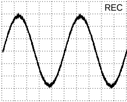
AC, 100mV/Div, 200µs/Div IC7601-(11) ⑨
