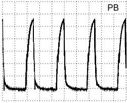
DC, 2V/Div, 5µs/Div T7330 - Gate 51
