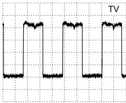
DC, 500mV/Div, 20µs/Div IC7200-(37), Connector 1922-(4) 33
