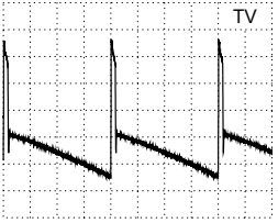
DC, 10V/Div, 5ms/Div IC7510-(5) 46
