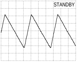
AC, 500mV/Div, 10µs/Div IC7310-(10) 52
