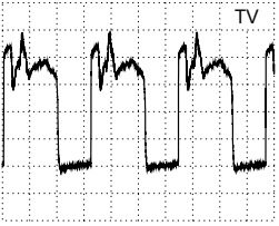
DC, 200mV/Div, 20µs/Div IC7584 - Basis 47
