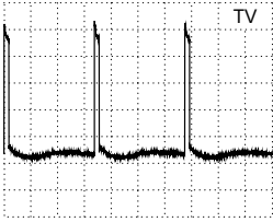
DC, 5V/Div, 5ms/Div IC7510-(8) 48
