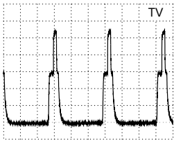
DC, 1V/Div, 20µs/Div IC7200-(38), Connector 1922-(5) 34
