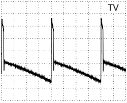
DC, 10V/Div, 5ms/Div T7584 - Basis 46
